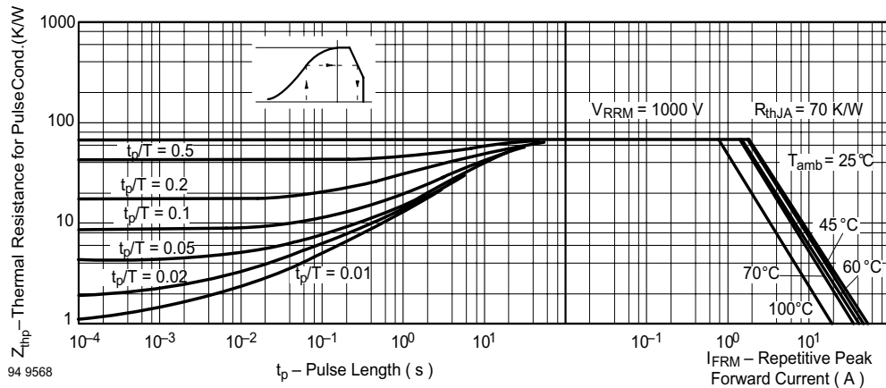
Figure 7. Thermal Response
